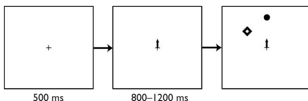
Fig. 1 Example of the display sequence. The arrow indicated the target location. After a variable delay, the target ('filled circle') and the distractor ('diamond shape') were presented simultaneously and observers were required to make a fast eye movement to the target. The distractor was presented on a third of the trials.
