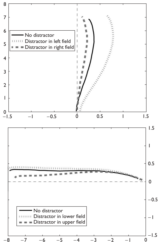
Fig. 3 Mean saccade trajectories for upward and leftward saccades for one observer. Both axes denote visual angle (deg).
